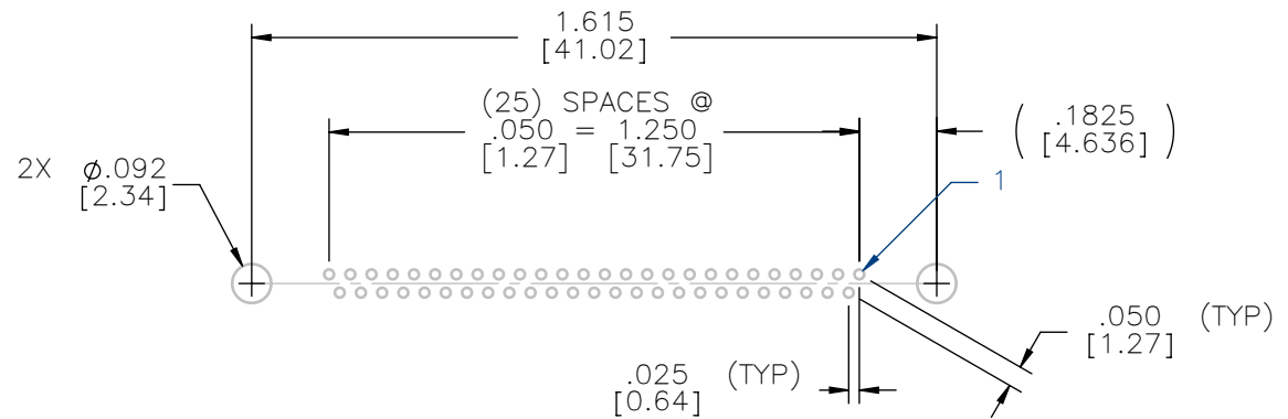
SUGGESTED HOLE PATTERN
