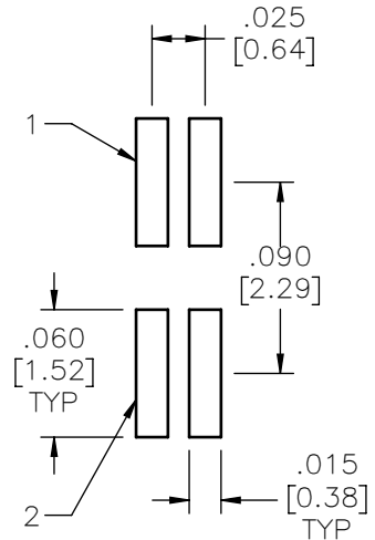
SUGGESTED PAD LAYOUT
