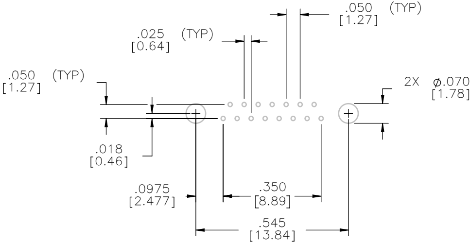
SUGGESTED HOLE PATTERN
