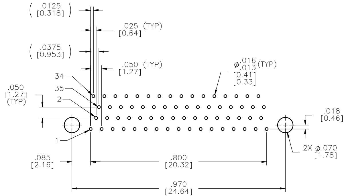
SUGGESTED HOLE PATTERN
