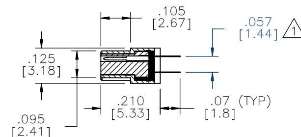
SECTION A-A VIEW LESS HARDWARE
