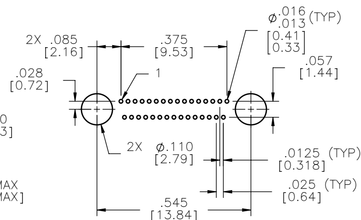
SUGGESTED HOLE PATTERN
