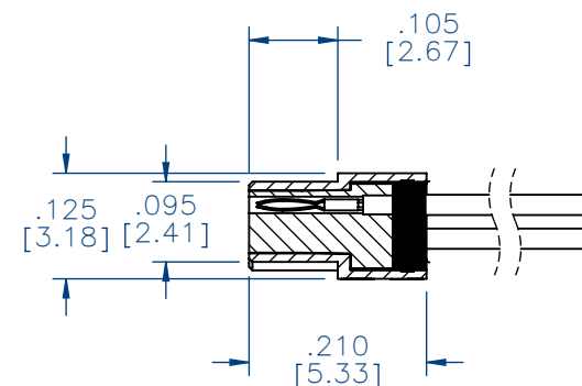
SECTION A-A VIEW LESS HARDWARE
